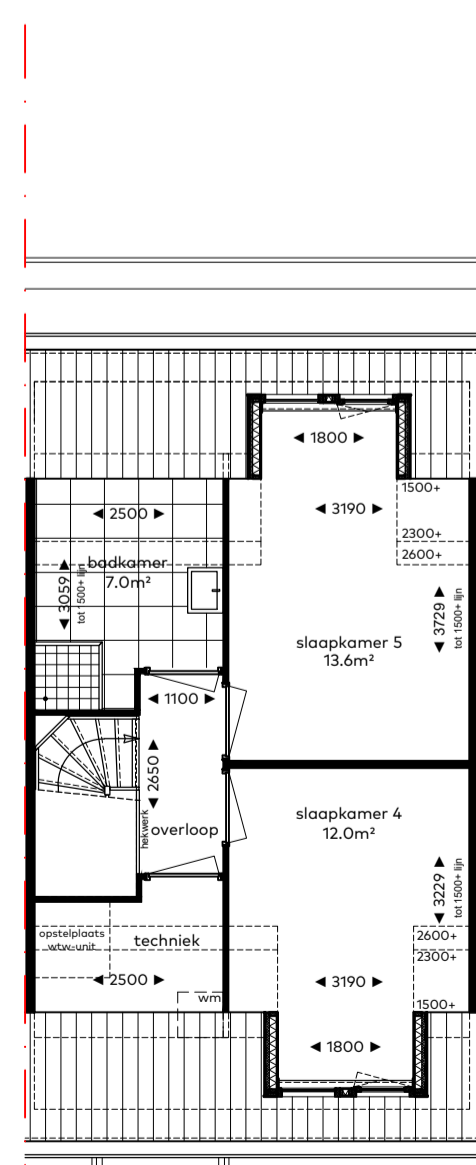
optie E-07 extra badkamer zolder
